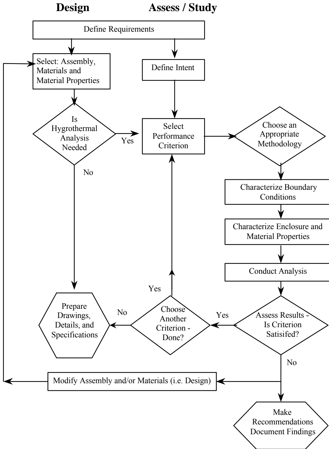
Figure 2: General Hygrothermal Enclosure Design or Assessment Procedure
